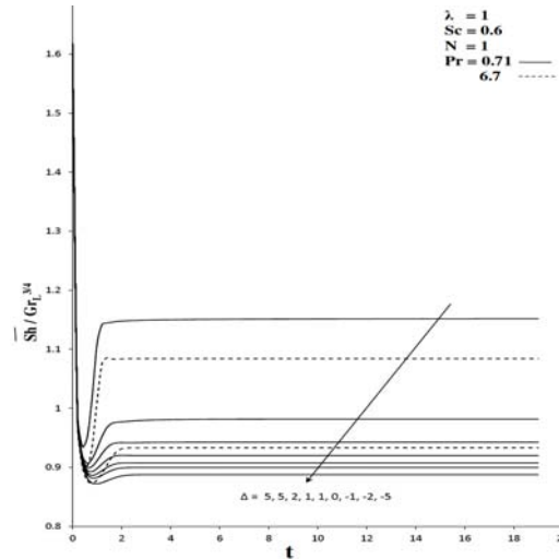
Fig. 7c. Average Sherwood Number for different values of Pr & \Delta in transient period.
