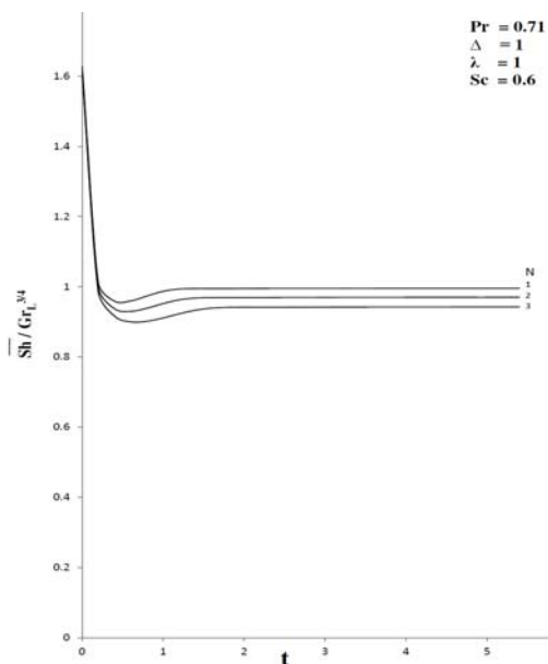
Fig. 9c. Average Sherwood number for different values of N in transient period.
