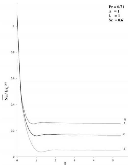
Fig. 9b. Average Nusselt Number for different values of N in transient period.
