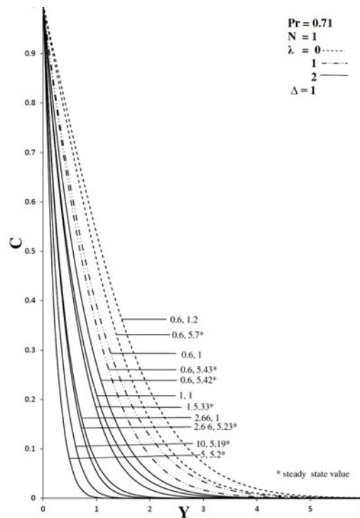
Fig. 2c. Transient concentration profile at X=1.0 for different values for Sc & \lambda .
