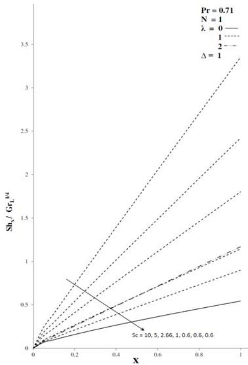
Fig. 5c. Local Sherwood Number for different values Sc & \lambda in transient state.
