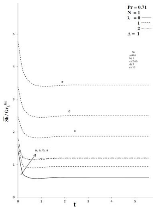
Fig. 8c. Average Sherwood number for different values of Sc & \lambda in transient period.
