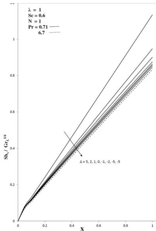
Fig. 4c. Local Sherwood Number for different values Pr & \Delta in transient state.
