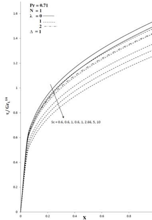
Fig. 5a. Local Skin Friction for different values Sc & \lambda in transient state.
