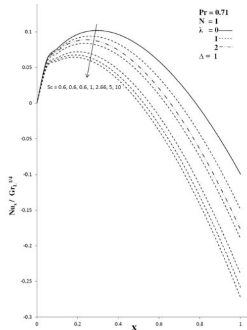
Fig. 5b. Local Nusselt Number for different values Sc & \lambda in transient state.
