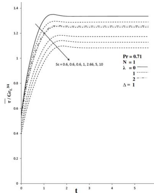
Fig. 8a. Average Skin Friction for different values of Sc & \lambda in transient period.
