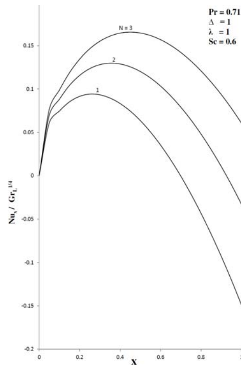
Fig. 6b. Nusselt Number for different values of N in transient period.
