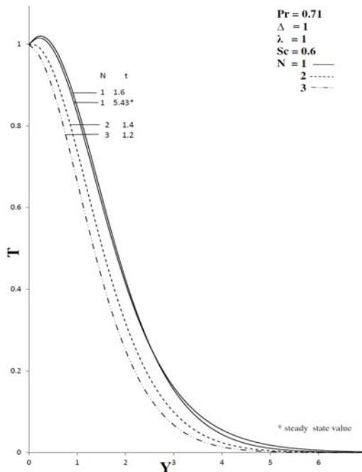
Fig. 3a. Transient temperature profiles at X=1.0 for different values for N .
