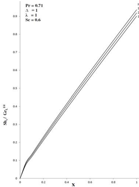
Fig. 6c. Local Sherwood number for different values of N in transient period.
