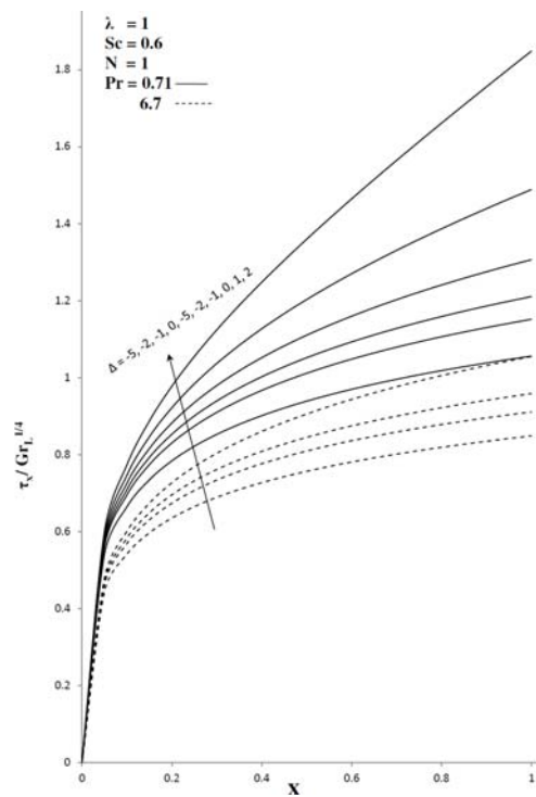
Fig. 4a. Local Skin Friction different values Pr & \Delta in transient state.
