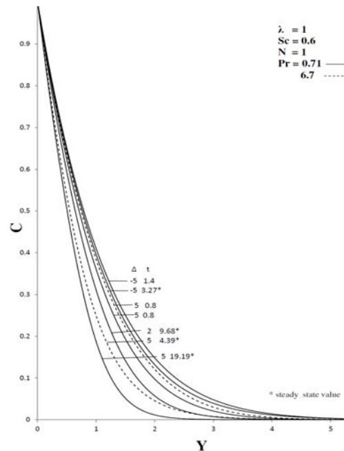
Fig. 1c. Transient concentration profile at X= 1.0 for different values for Pr & Δ.
