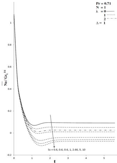
Fig. 8b. Average Nusselt Number for different values of Sc & \lambda in transient period.
