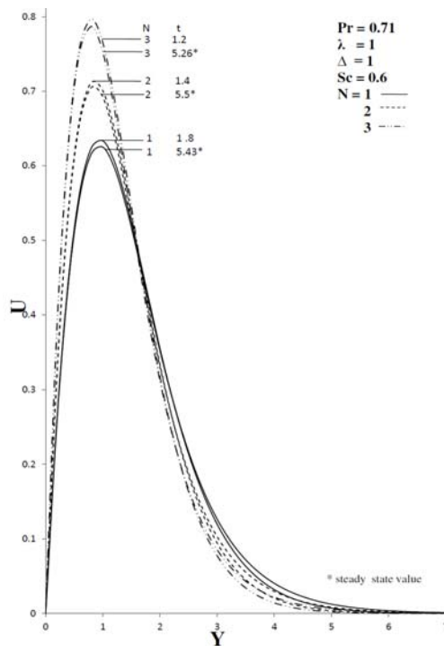
Fig. 3b. Transient velocity profiles at X=1.0 for different values for N .
