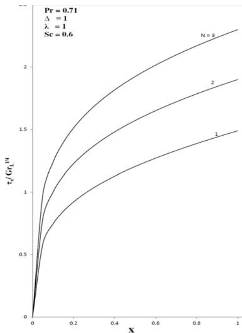
Fig. 6a. Local Friction for different values of N in transient period.
