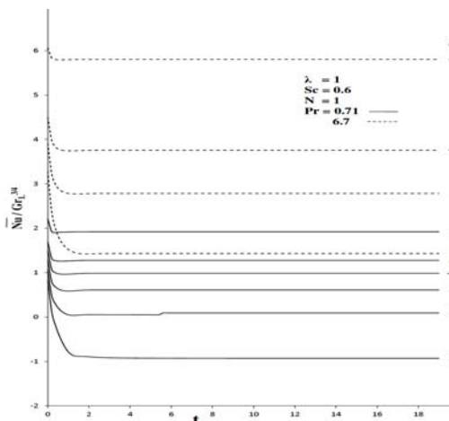
Fig. 7b. Average Nusselt Number for different values of Pr & D & m in transient period.
