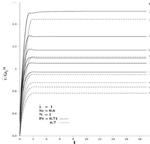
Fig. 7a. Average Skin Friction for different values of Pr & \Delta in transient period.
