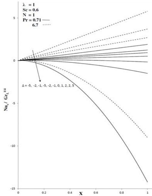
Fig. 4b. Local Nusselt Number for different values Pr & \Delta in transient state.
