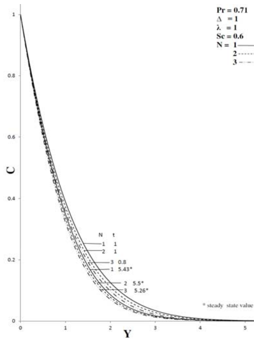
Fig. 3c. Transient concentration profiles at X=1.0 for different N .
