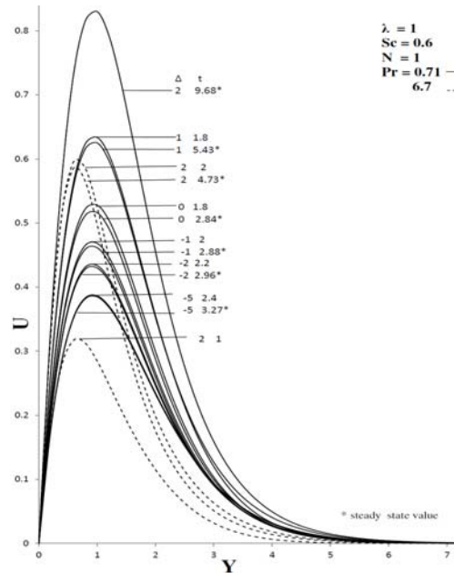
Fig. 1b. Transient Velocity profile at X= 1.0 for different values for Pr & Δ.
