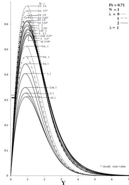
Fig. 2b. Transient t Velocity profiles at X=1.0 for different values for Sc & \lambda .
