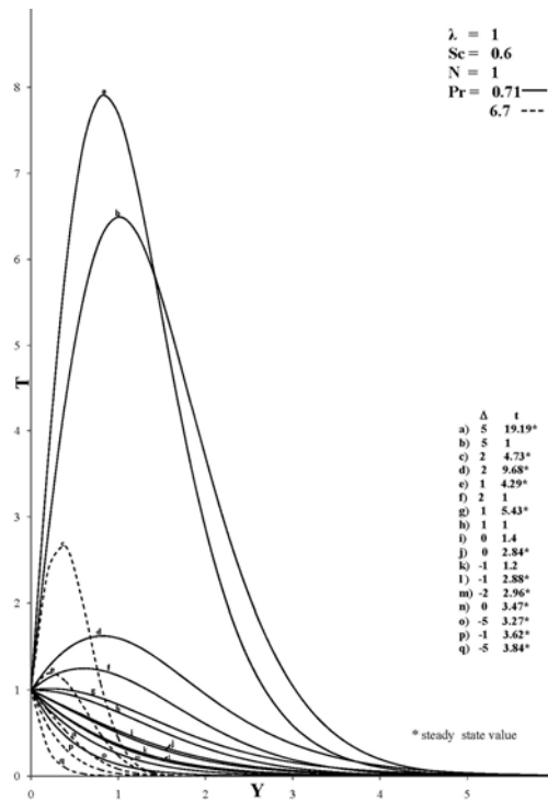
Fig. 1a. Transient Temperatur profils at X=1.0 for different values for Pr & Δ.
