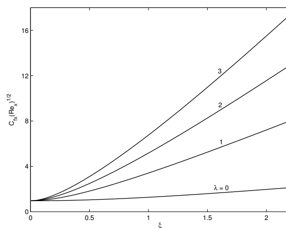
Fig. 17 Effect of \lambda on C_{fx}(Re_x)^{1/2} when A = 0.0 , m = 0.0909 , n = 1.0 , Pr = 0.72 , S = 1.0 , M = 0.1 , K = 0.1 , Sc = 0.62 and \Delta = 1.0 .
