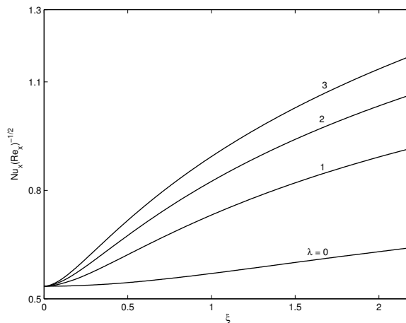
Fig. 18 Effect of \lambda on Nu_x(Re_x)^{-1/2} when A = 0.0 , m = 0.0909 , n = 1.0 , Pr = 0.72 , S = 1.0 , M = 0.1 , K = 0.1 , Sc = 0.62 and \Delta = 1.0 .
